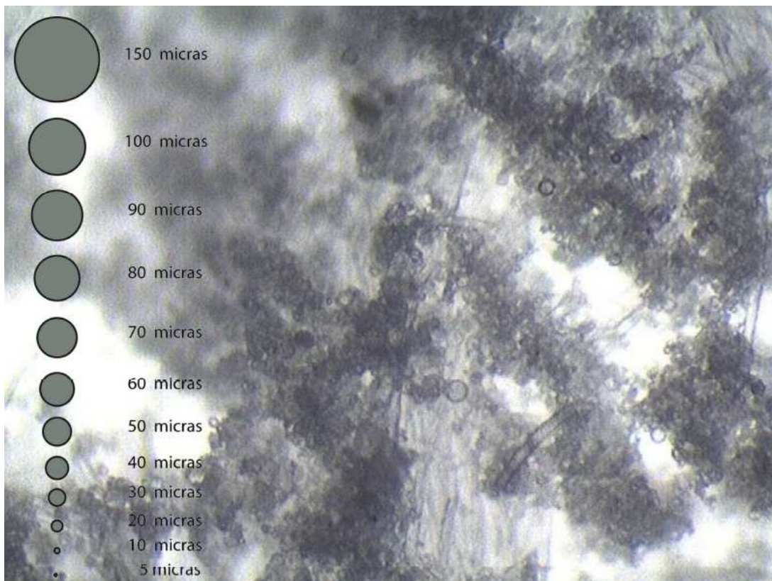
Picture of the fabric with microspheres collected after filtration
